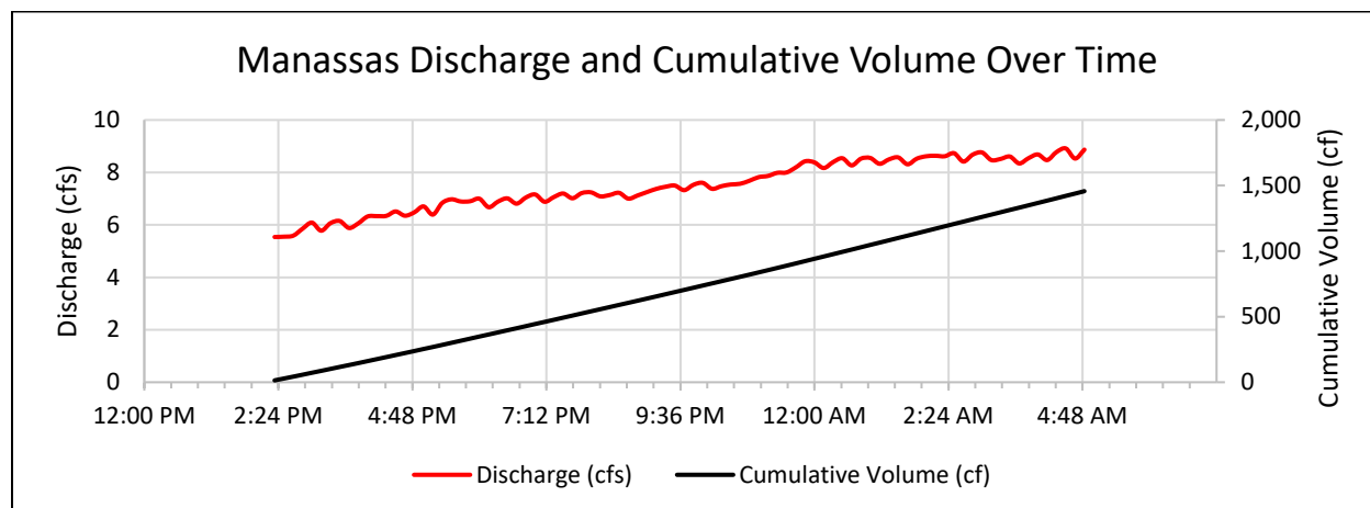
Figure 1: Flow data over time for the storm event at Site #941 on November 14 - 15, 2024
