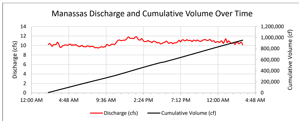
Figure 1: Flow data over time for the storm event at Site #941 on January 30 – February 1, 2025
