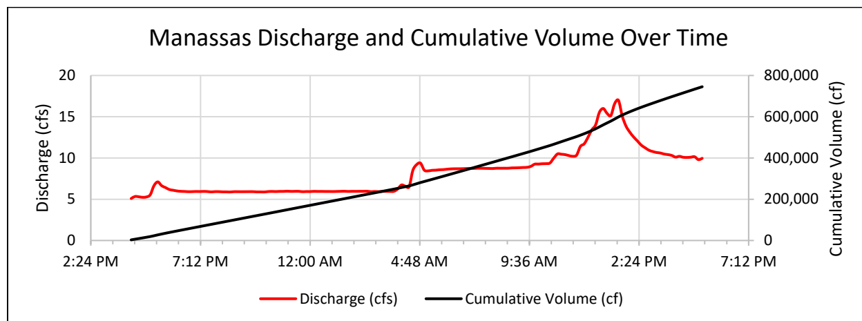
Figure 1: Flow data over time for the storm event at Site #941 on September 17 - 18
