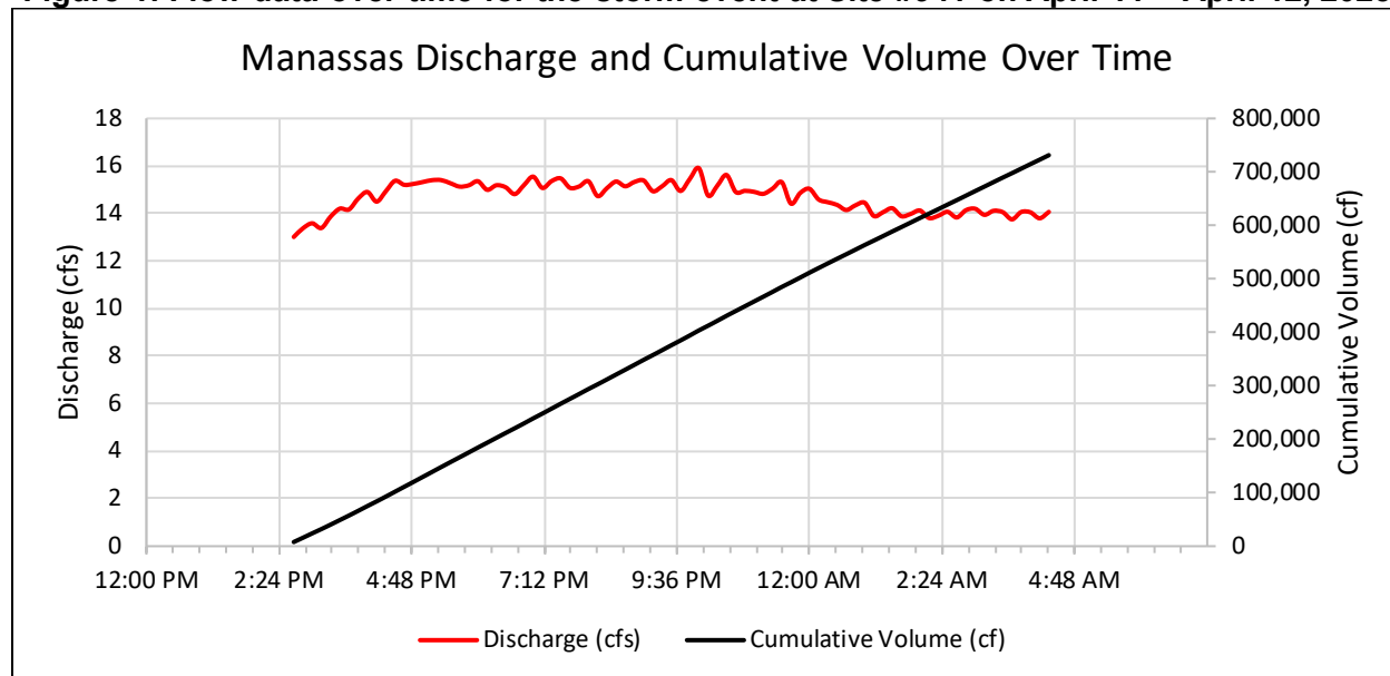
Figure 1: Flow data over time for the storm event at Site #941 on April 11 – April 12, 2025
