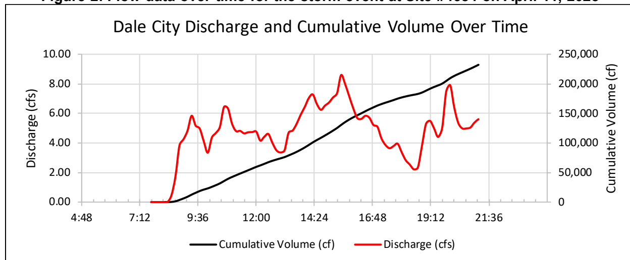
Figure 2: Flow data over time for the storm event at Site #4684 on April 11, 2025
